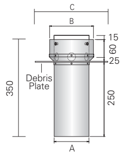
Turboflex Plus Adaptor & Debris Plate
