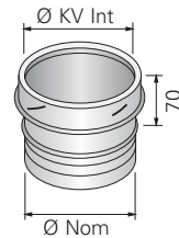
Adaptor to K-Vent
