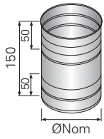
Double Male Adaptor
