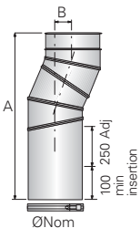
0-90° Adjustable Bend Extendable P+ S084 P+1 S184
