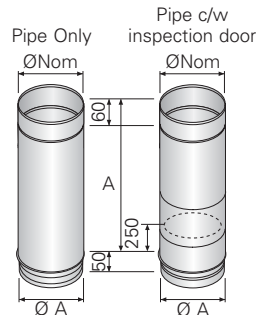
Imperial Starter Pipe
