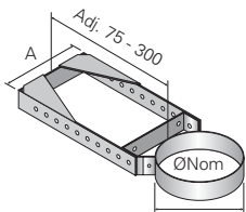
Wall Bracket 300mm Adjustable 95960
