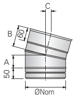
15° Bend P+ S018 P+1 S118
