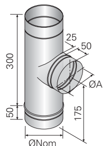
90° Starter Tee Imperial
