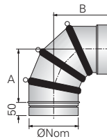
0-90° Adjustable Bend Condensing P+ S006 P+1 S106
