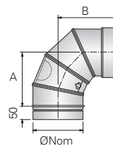
0-90° Adjustable Bend Inspection Standard P+ S028 Extendable P+1 S0B1 P+1 S128 P+1 S1B1
